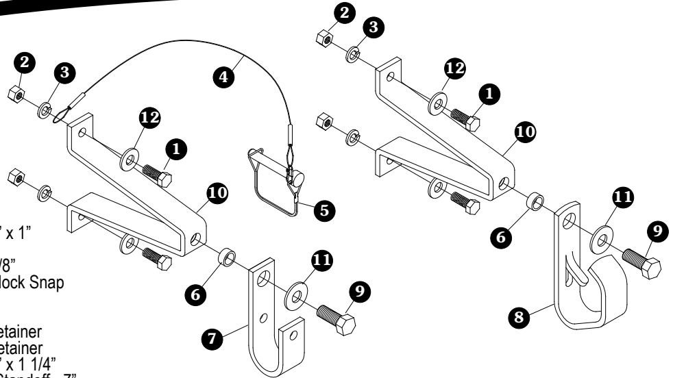
Stainless Steel J-Hook Crank Retainer
