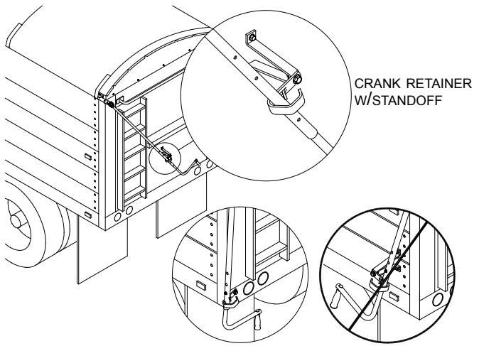
CRANK RETAINER W/STANDOFF CRANK RETAINER WITHOUT STANDOFF DO NOT MOUNT CRANK RETAINER ON SIDE OF BOX
