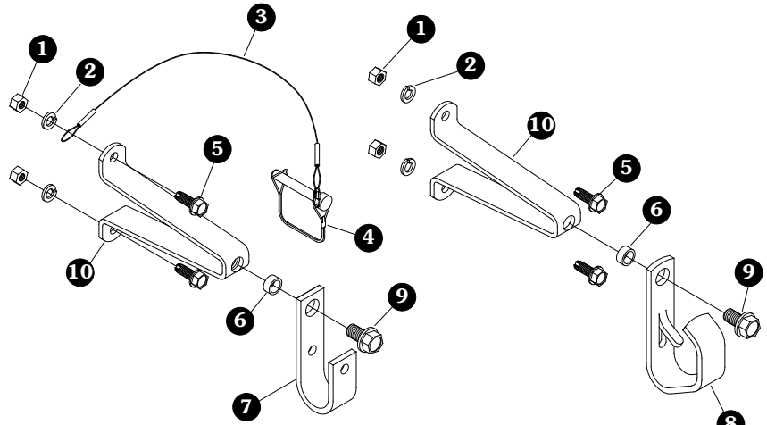
J-Hook Crank Retainer
