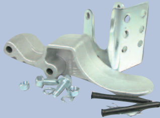
1111094 EO Aluminum Tarp Stop Assembly
