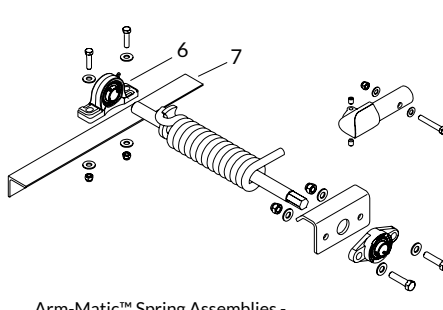
Arm-Matic™ Spring Assemblies - Underbody Hex/Round Shaft
