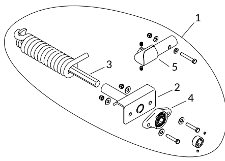
Arm-Matic™ Spring Assemblies - Underbody Hex Shaft
