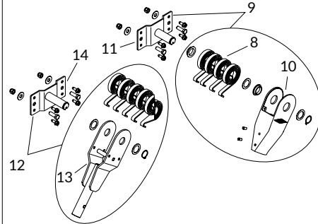
Arm-Matic™ Spring Assemblies - External Pivot
